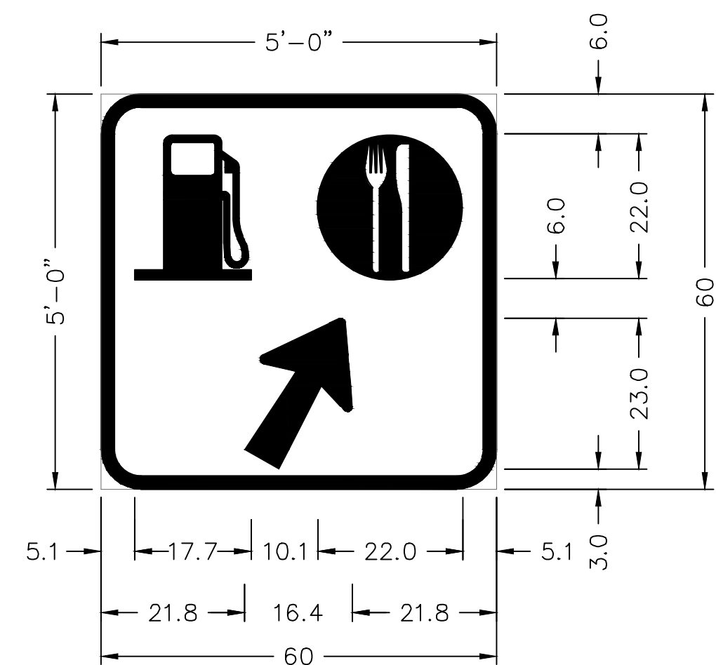
MPT-08 2.0" Border With 6.0" Radius White on Blue
