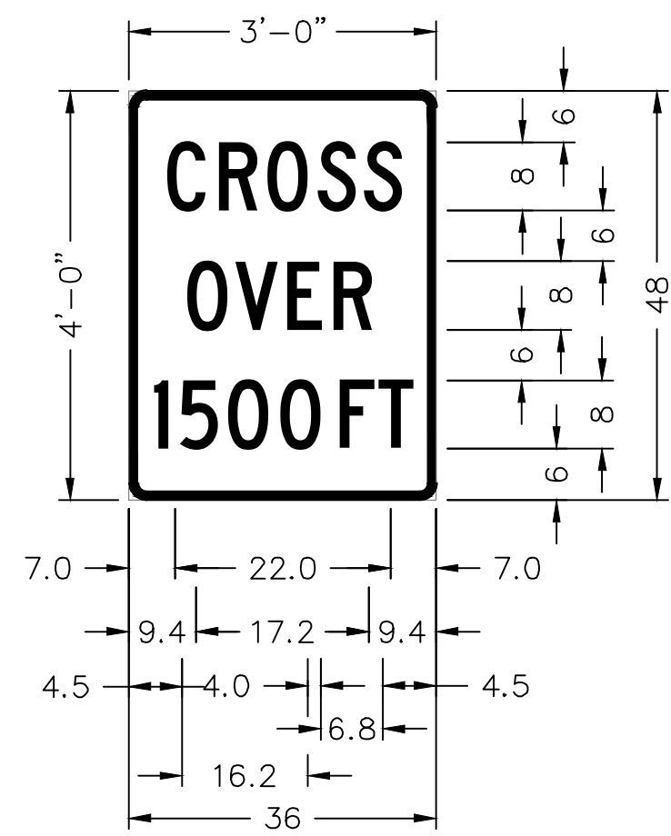
MPT-03 1.0" Border With 2.0" Radius Black on Orange
