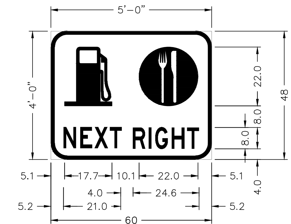
MPT-07 1.3" Border With 6.0" Radius White on Blue
