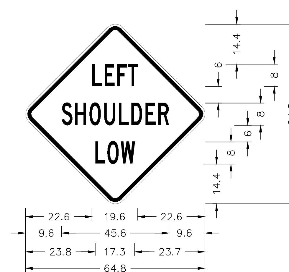
MPT-38 48" Across Sides, 0.8" Border, 0.4" Indent With 3.8" Radius Black on Orange
