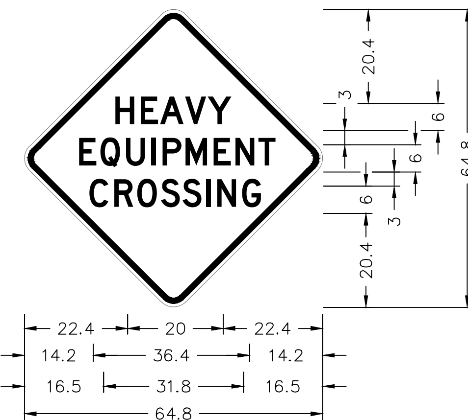
MPT-36 48" Across Sides, 0.8" Border, 0.4" Indent With 3.8" Radius Black on Orange
