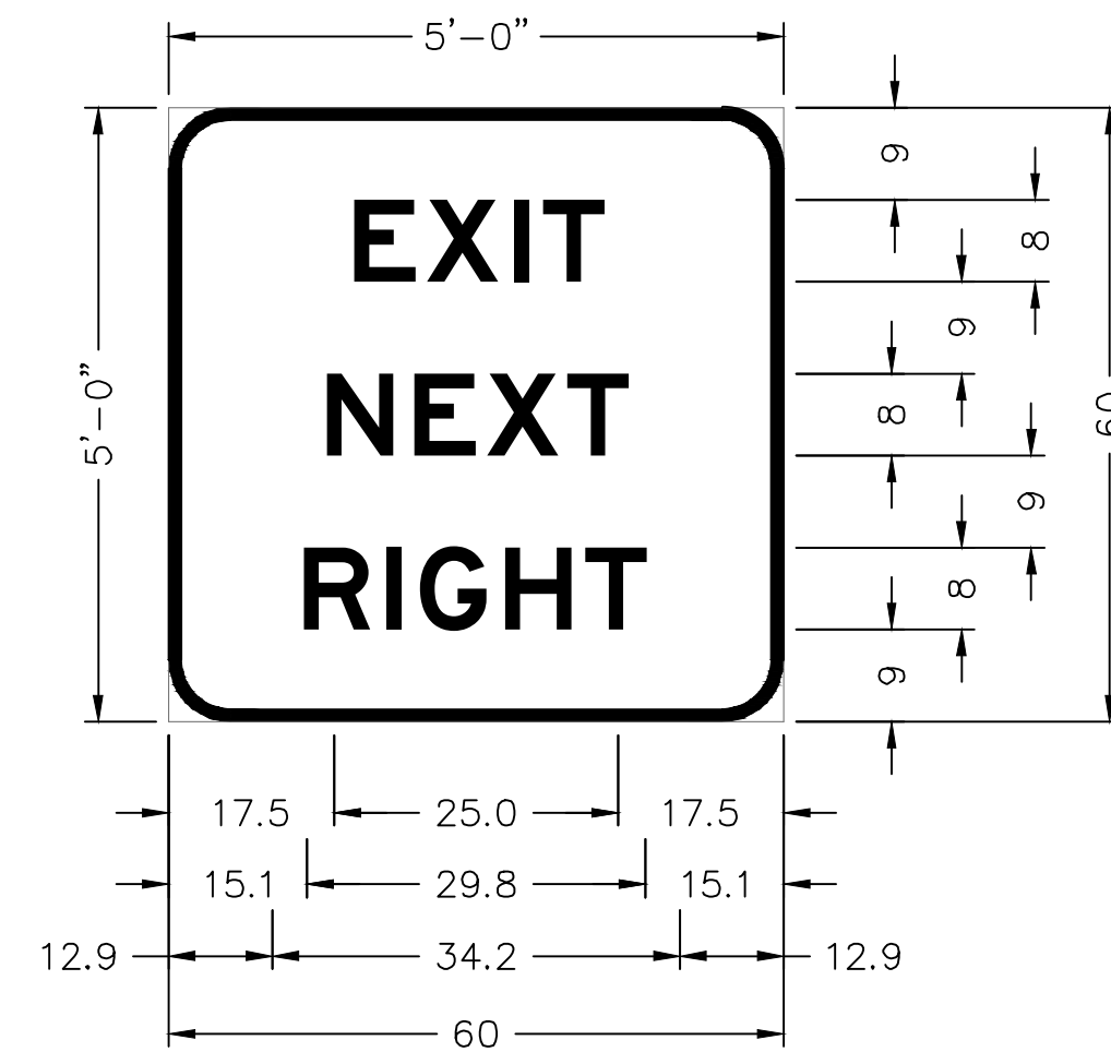
MPT-05 1.3" Border With 6.0" Radius White on Green
